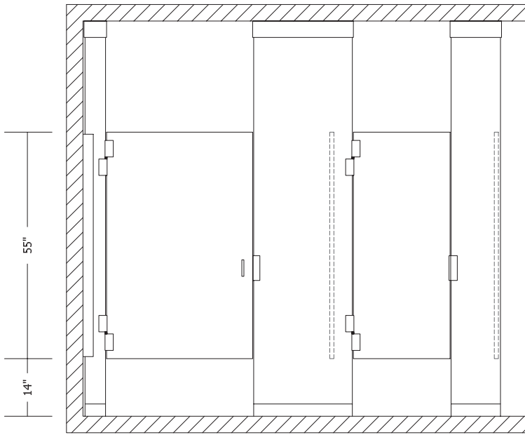
STANDARD FRONT ELEVATION
