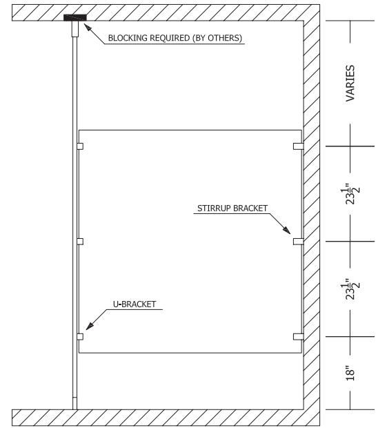
STANDARD SIDE ELEVATION WITH BLOCKING LOCATIONS
