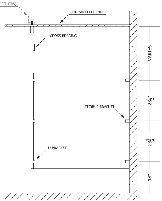
STANDARD SIDE ELEVATION WITH BLOCKING LOCATIONS
