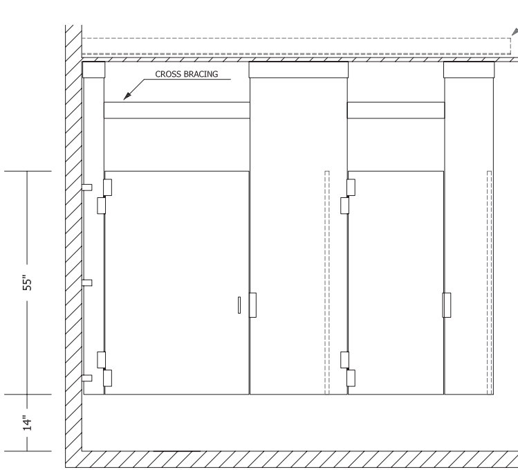
STANDARD FRONT ELEVATION
